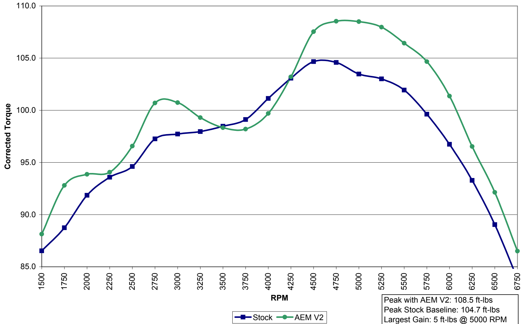
01-03 Honda Civic EX With AEM V2 Corrected Torque
